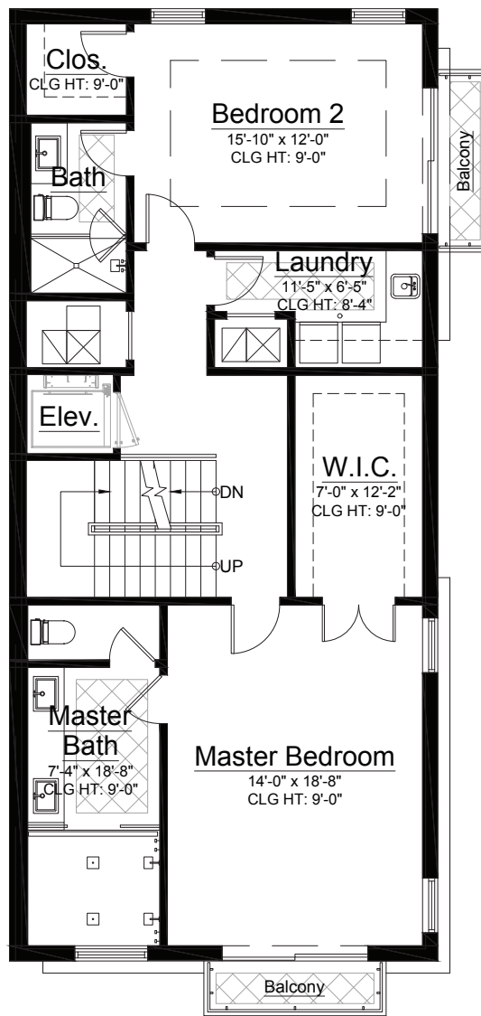
SECOND FLOOR
