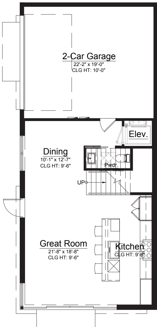
FIRST FLOOR
