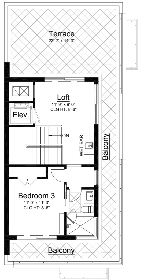
THIRD FLOOR
